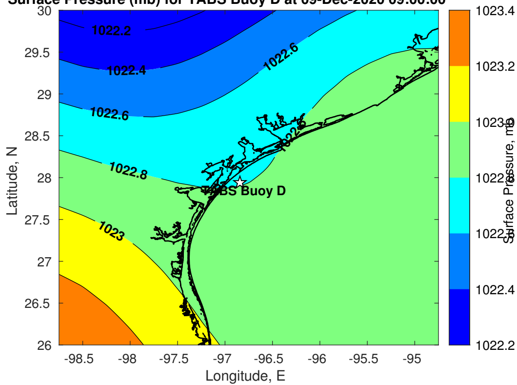
Surface Pressure (mb) for TABS Buoy D at 09-Dec-2020 09:00:00
