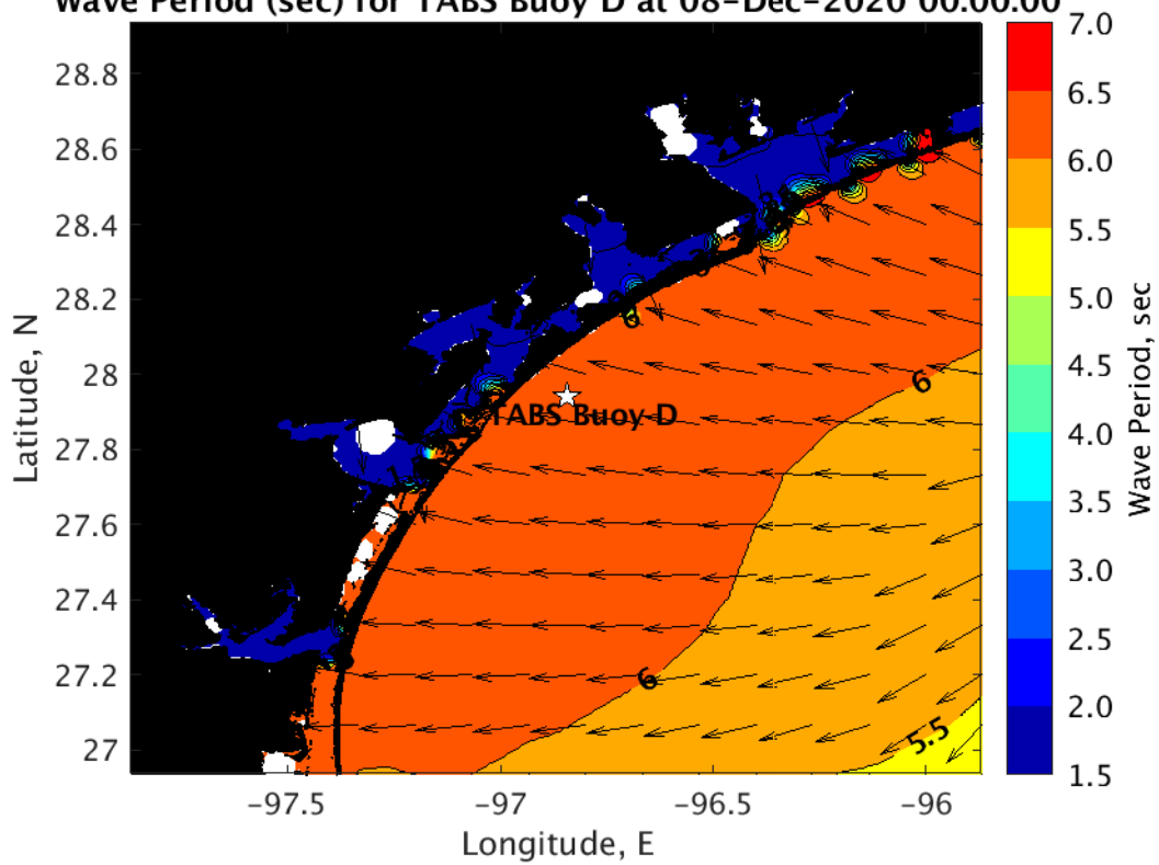
Wave Period (sec) for TABS Buoy D at 08-Dec-2020 00:00:00
