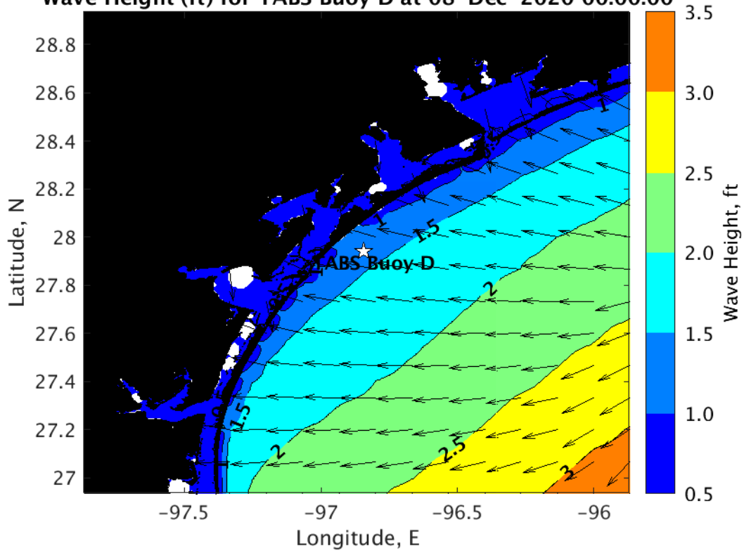
Wave Height (ft) for TABS Buoy D at 08-Dec-2020 00:00:00
