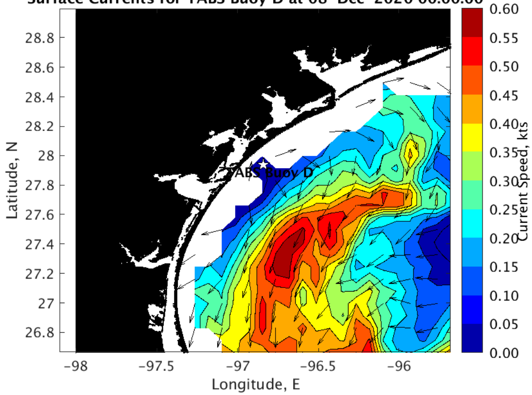
Surface Currents for TABS Buoy D at 08-Dec-2020 00:00:00
