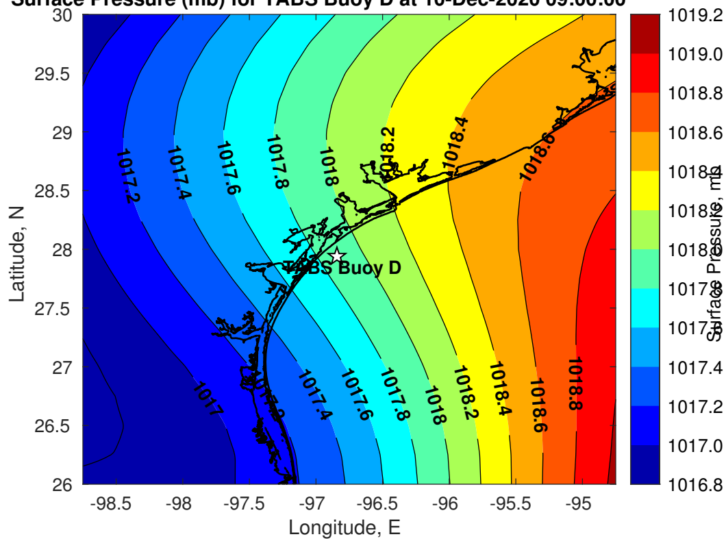
Surface Pressure (mb) for TABS Buoy D at 10-Dec-2020 09:00:00
