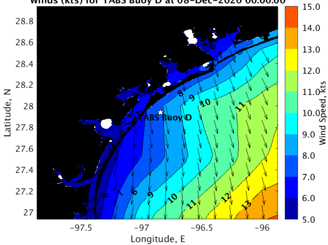
Winds (kts) for TABS Buoy D at 08-Dec-2020 00:00:00
