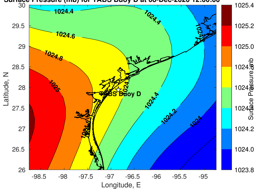
Surface Pressure (mb) for TABS Buoy D at 08-Dec-2020 12:00:00
